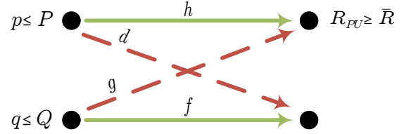
Fig. 1. A simple underlay CR scenario modeled as a two-user SISO-IC. The SU (bottom link) may transmit improper signals, but must guarantee the rate constraint of the PU (top link).
